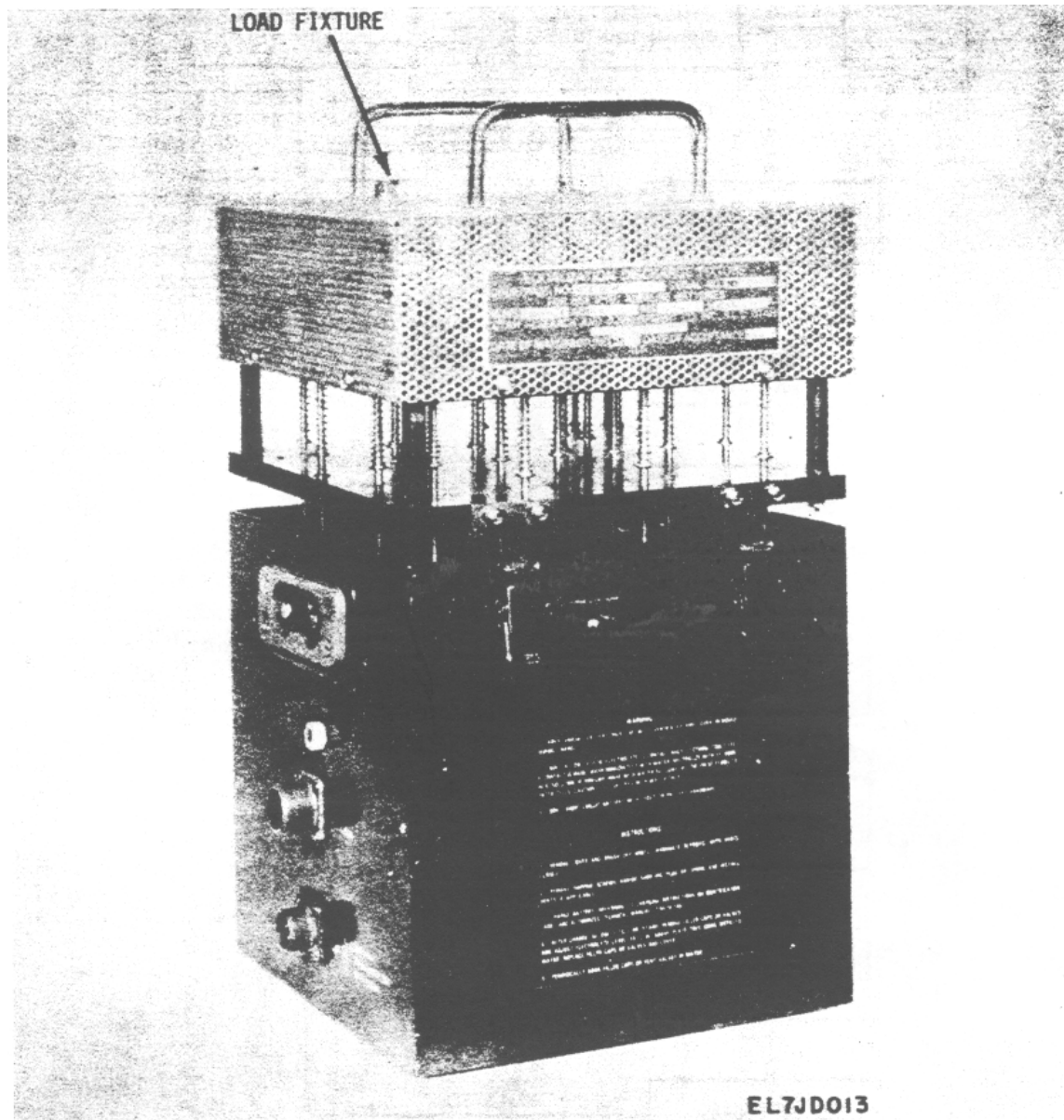
Figure 5-4. Discharging Battery.
